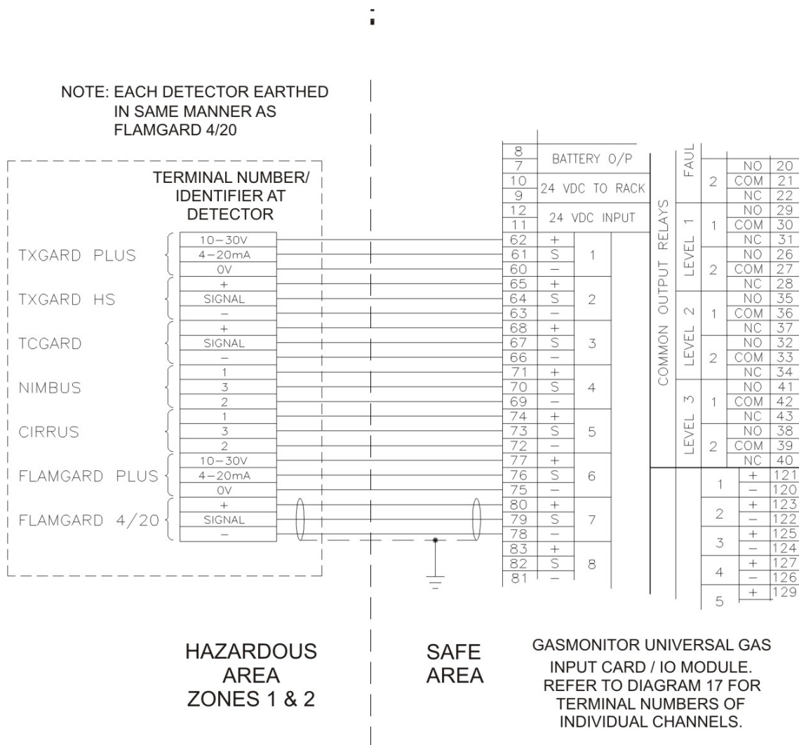
Figure 30: Gasmonitor+ to 3-wire 4-20 mA type detectors
