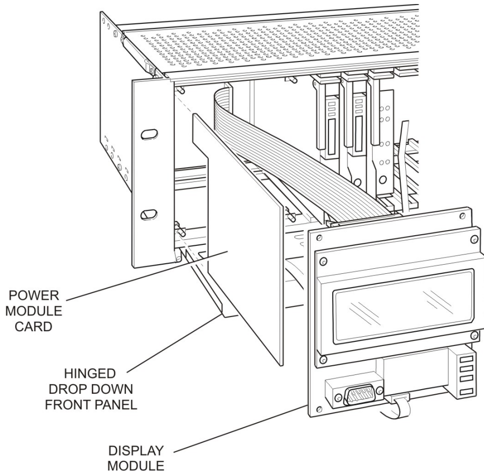
Figure 25: Power Module Mounting Detail
